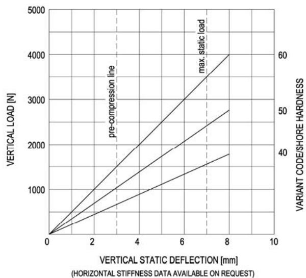
LOAD CHARACTERISTICS
