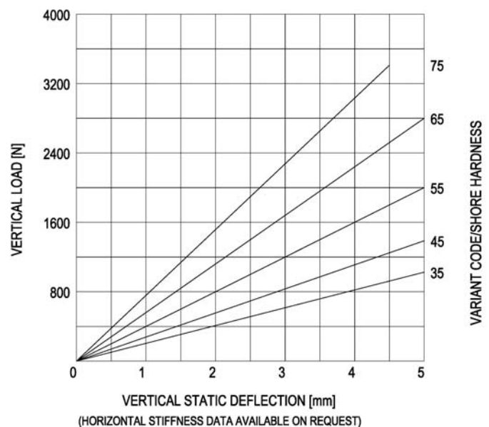
LOAD CHARACTERISTICS
